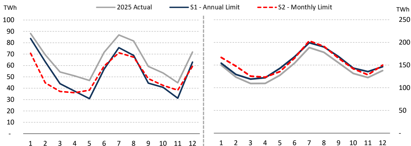
EXHIBIT 4 – MONTHLY LOWER-48 ACTUAL & MODELED 2025 COAL (LEFT) AND NATURAL GAS (RIGHT) GENERATION
