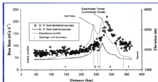
FIGURE 3: Variability of terrestrial and cosmic radiation background across the interstate 70 corridor of Colorado.*
